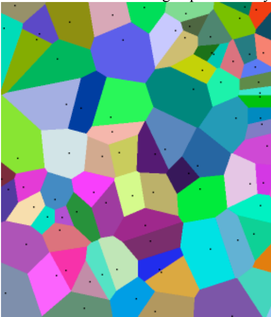
Figure 3. Example of a Voronoi partition of a set of points in two dimensions.
